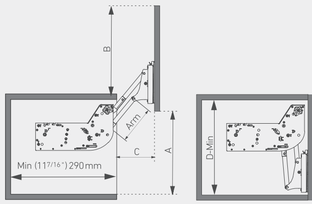
Cabinet & lift arm comparison
